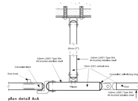
plan detail A-A
