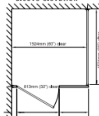
barrier-free plan
