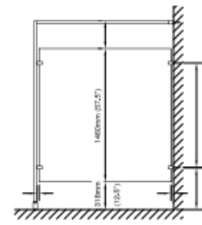
side elevation
